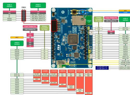
Figure 3: B-L475E-IOT01A Discovery Board pinout.
