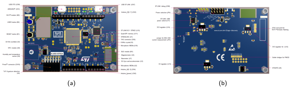
Figure 2: B-L475E-IOT01A top (a) and bottom (b) views.
