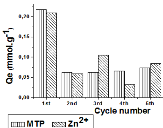
Figure 9. Adsorption capacity of 2-CS/1.5 MGO beads towards Zn^{2+} and MTP after a few cycles of regeneration.
