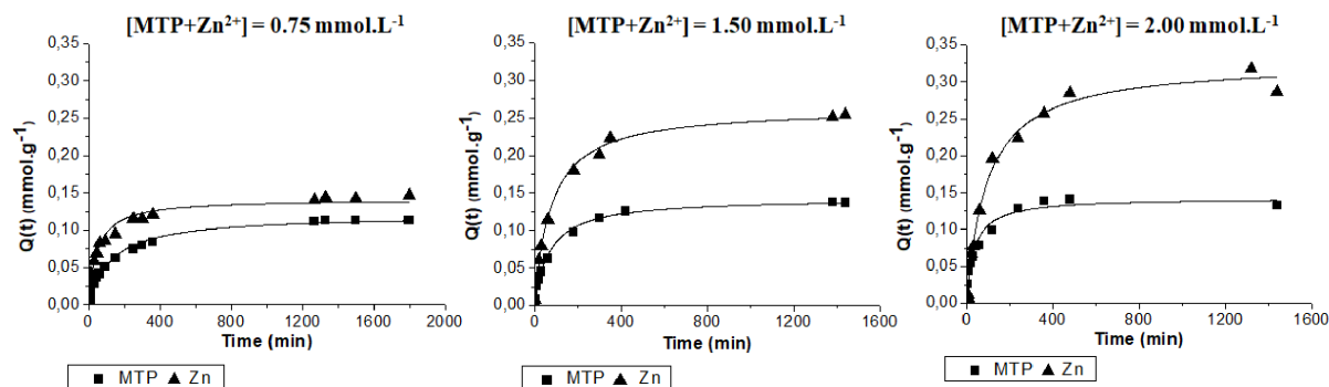
Figure 7. Adsorption kinetics of MTP and Zn^{2+} on 2-CS/1.5MGO beads in an MTP- Zn^{2+} equimolar mixture at different initial concentrations. The continuous lines represent calculated data using the best-fitting model.
