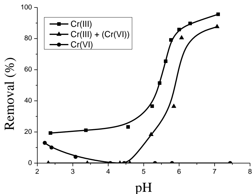
Figure 3. Effect of pH on Cr (III) removal by kaolinite ( C_{0(\text{Cr(III)})} : 10 mg/L, C_{0(\text{Cr(VI)})} : 10 mg/L, t: 60 min, kaolinite dose:1g/L)
