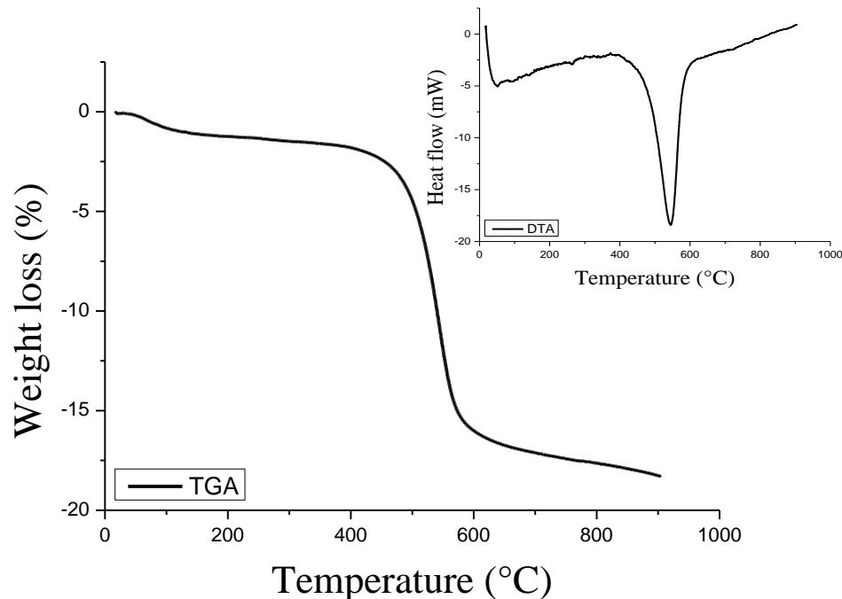
Figure 2. Thermal analysis of the raw kaolinite
