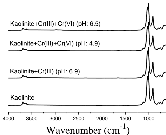
Figure 5. ATR-FTIR spectra of kaolinite after chromium adsorption
