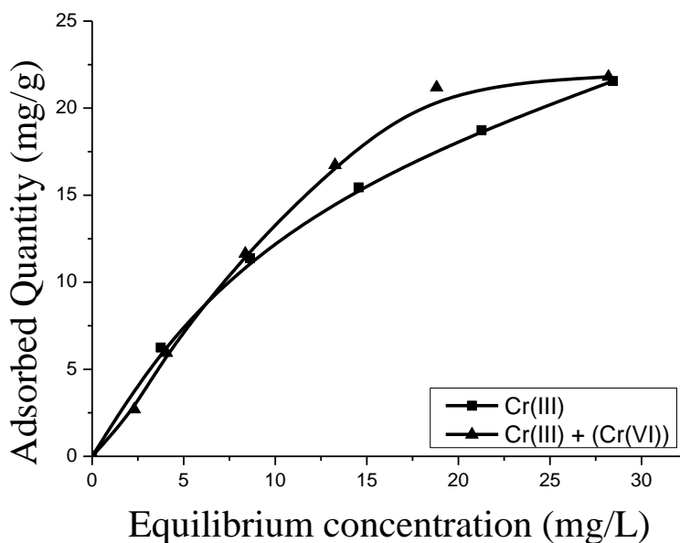
Figure 8. Isotherm of Cr (III) adsorption on kaolinite (kaolinite dose: 1 g/L, C_{0(\text{Cr(VI)})} : 10 mg/L, pH: 5, t: 24 h)
