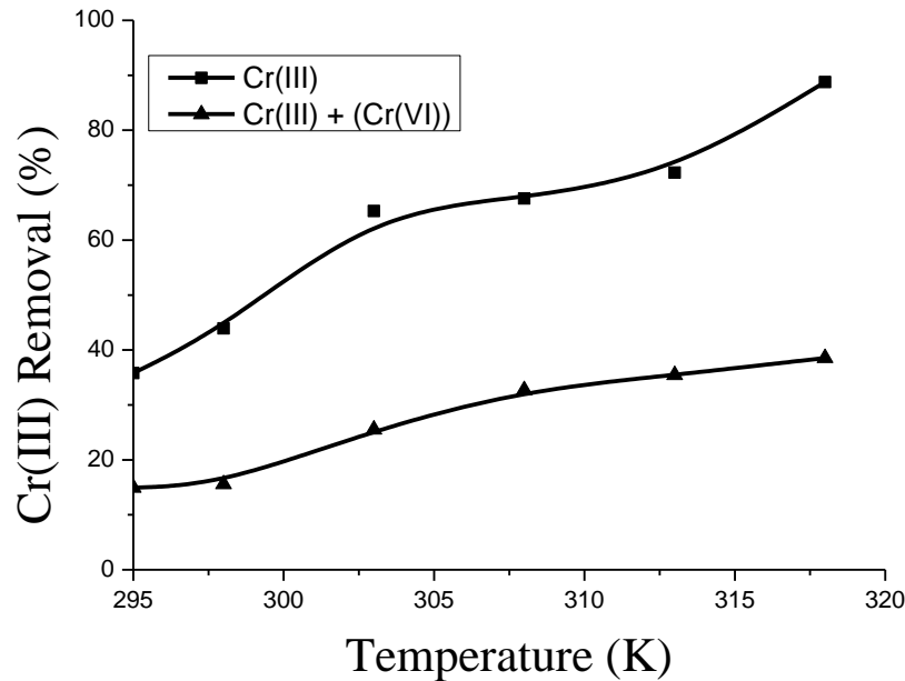
Figure 6. Effect of temperature on Cr (III) adsorption on kaolinite ( C_{0(\text{Cr(III)})} :10 mg/L, C_{0(\text{Cr(VI)})} : 10 mg/L, kaolinite dose:1 g/L, pH: 5, t: 60 min)
