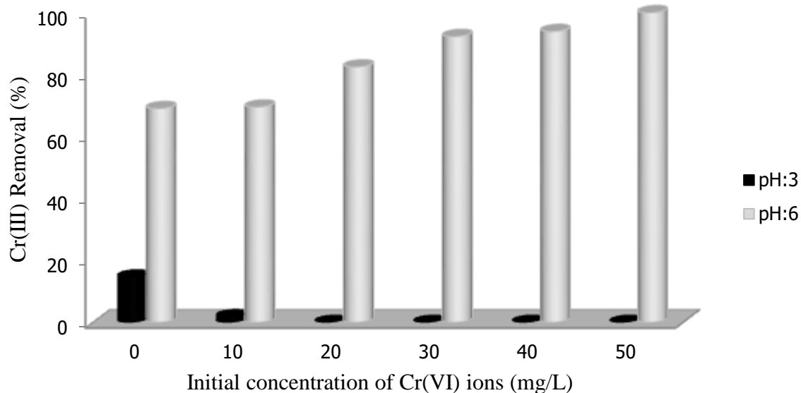
Figure 4. Effect of increasing Cr(VI) concentration on Cr(III) adsorption on kaolinite ( C_{0(Cr(III))} : 10 mg/L, kaolinite dose: 1 g/L, t: 60 min)
