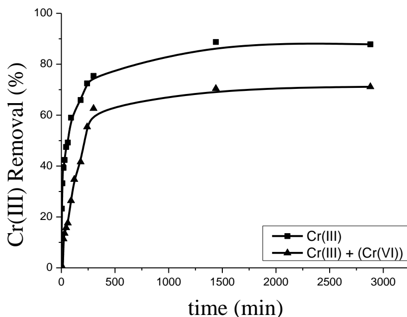
Figure 7. Effect of time on Cr (III) adsorption on kaolinite
