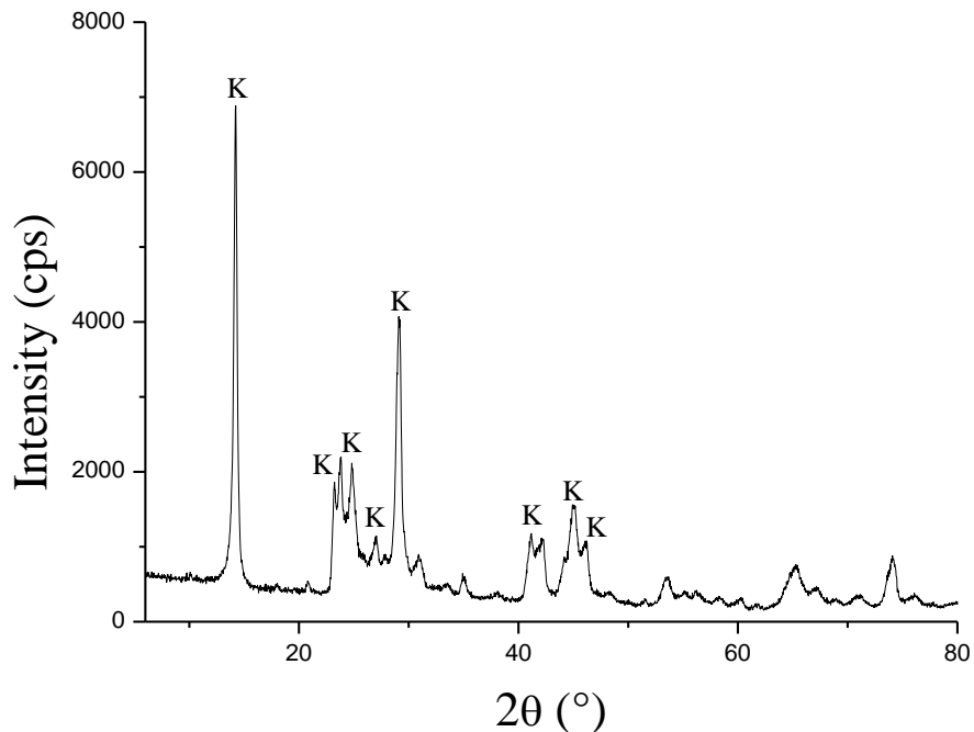
Figure 1. X-ray diffraction spectrum of the pristine kaolinite
