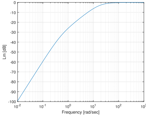
Fig. 6. Log-magnitude plot of M (vide small-gain theorem)
