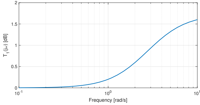
Fig. 7. Complementary sensitivity function T_1(j\omega) for \overline{f_{xy}} = 4 , k_p = 25 , k_v = 10
