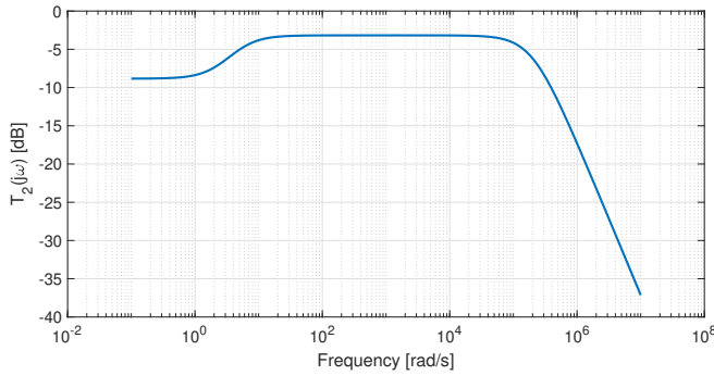
Fig. 8. Complementary sensitivity function T_2(j\omega) for \overline{f_{xy}} = 4 , k_p = 25 , k_v = 10
