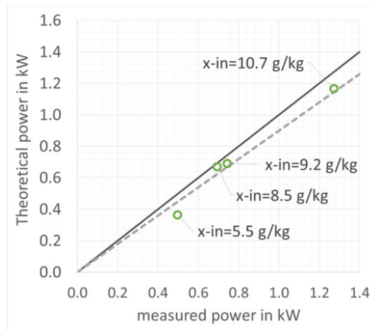
Fig. 10: Thermal power delivered to the heating system as a function of the theoretical thermal power
