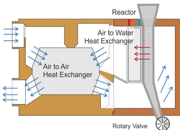
Fig. 9: Reactor unit of the sorption storage: discharging mode
